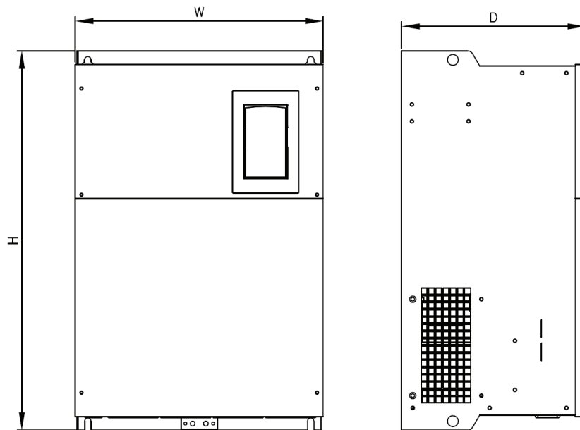
Frame 6, 7, 8, 9, 10, 11 (IP20)
